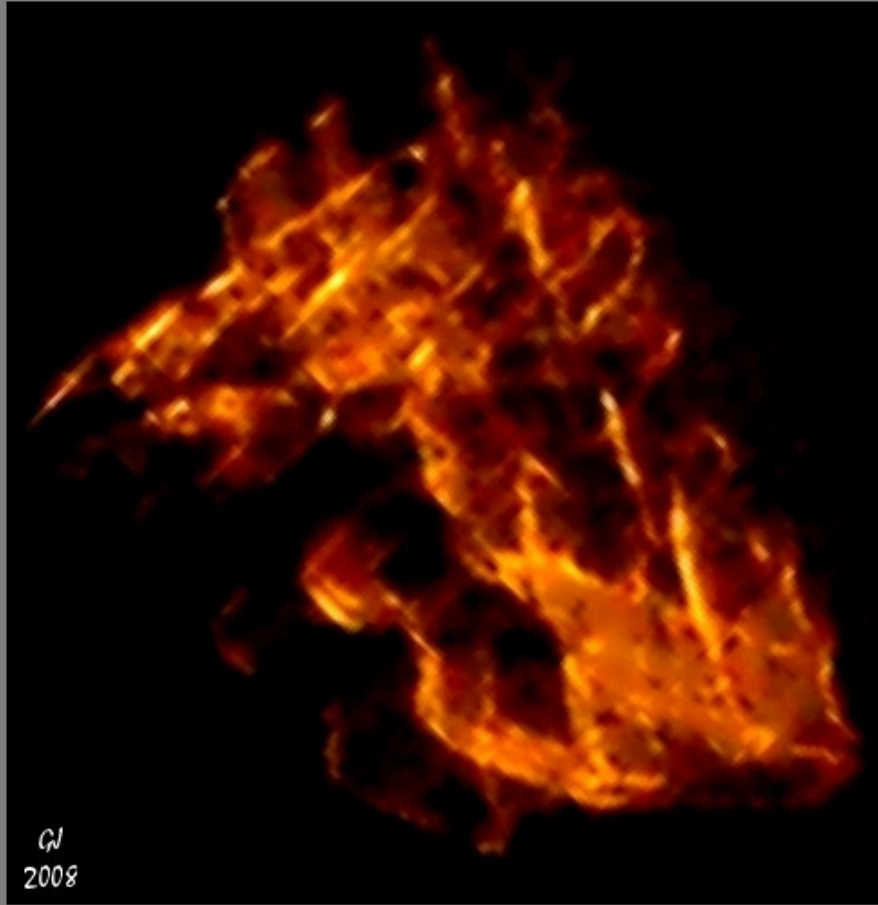
charmed hadron
