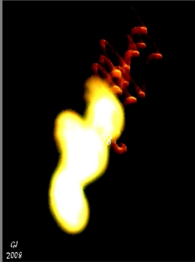
lepton of definite charge
