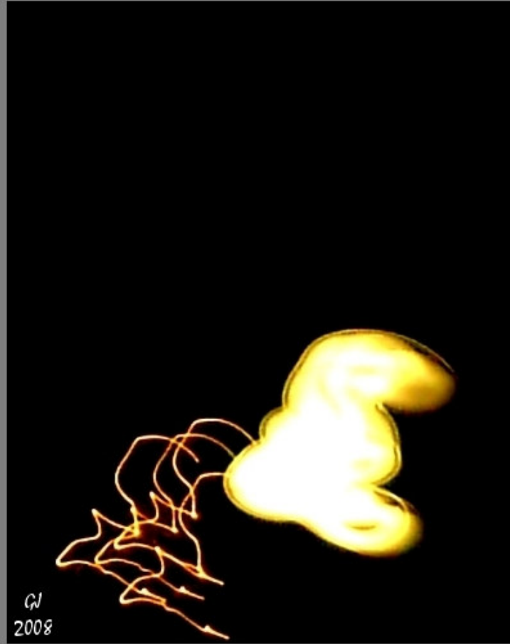
strange quark
